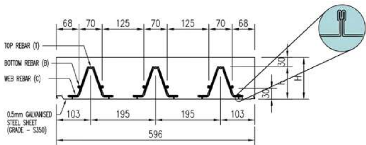
Enviro Deck a Section
