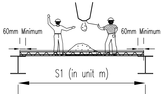
Unpropped Steel Construction for Single Span Enviro Deck
