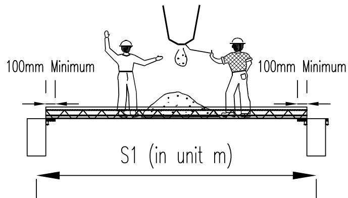
Unpropped RC Construction for Single Span Enviro Deck
