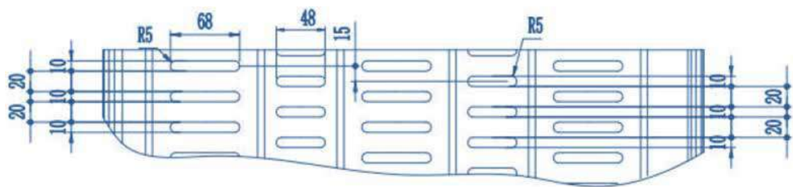
Enviro Deck Plan view with Embossment
