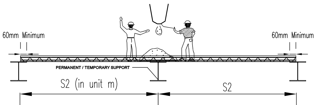
Propped Steel Construction for Continuous Span Enviro Deck
