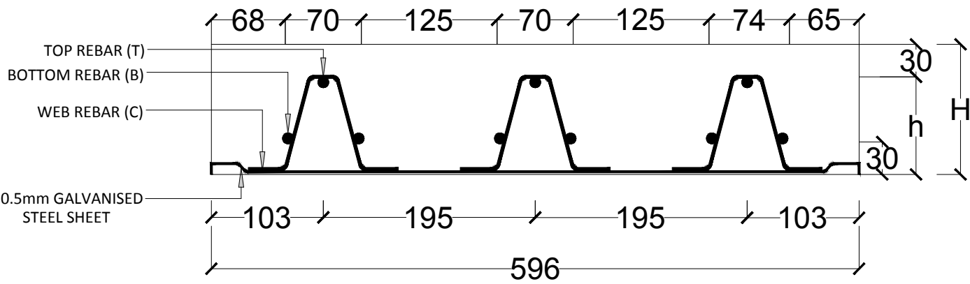
Enviro Deck a Section
