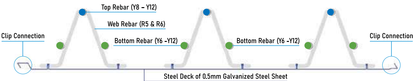
Enviro Deck a Profile with Prefab. Rebar
