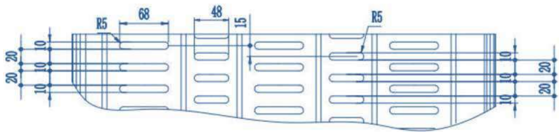
Enviro Deck a Plan view with Embossment
